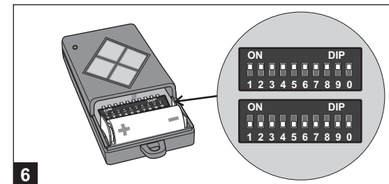
1/4-Kanal Handsender Linear-Code, mit Kodierschalter 1/4-channel handheld transmitter Linear code, with coding switch S10-433A1L01 / S10-433A4L01 S10-868A1L01 / S10-868A4L01
