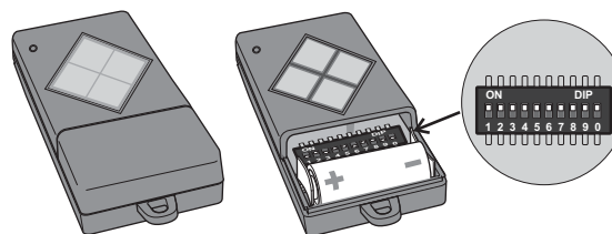
1/4-Kanal Handsender Linear-Code, mit Kodierschalter 1/4-channel handheld transmitter Linear code, with coding switch S10-433A1L01 / S10-433A4L01 S10-868A1L01 / S10-868A4L01
