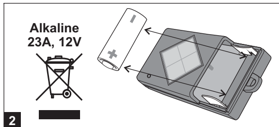
1/4-Kanal Handsender KeeLoq, Hopping / Wechsel-Code 1/4-channel handheld transmitter KeeLoq, hopping/change code S10-433A1K01 / S10-433A4K01 S10-868A1K01 / S10-868A4K01
